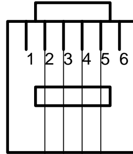
telephone modular plug 6p
