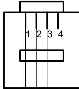
telephone modular plug 4p
